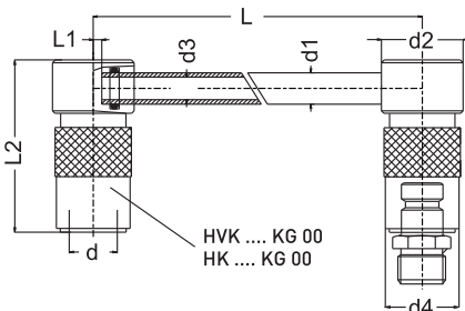
Diverging connector / Umlenkkupplung
